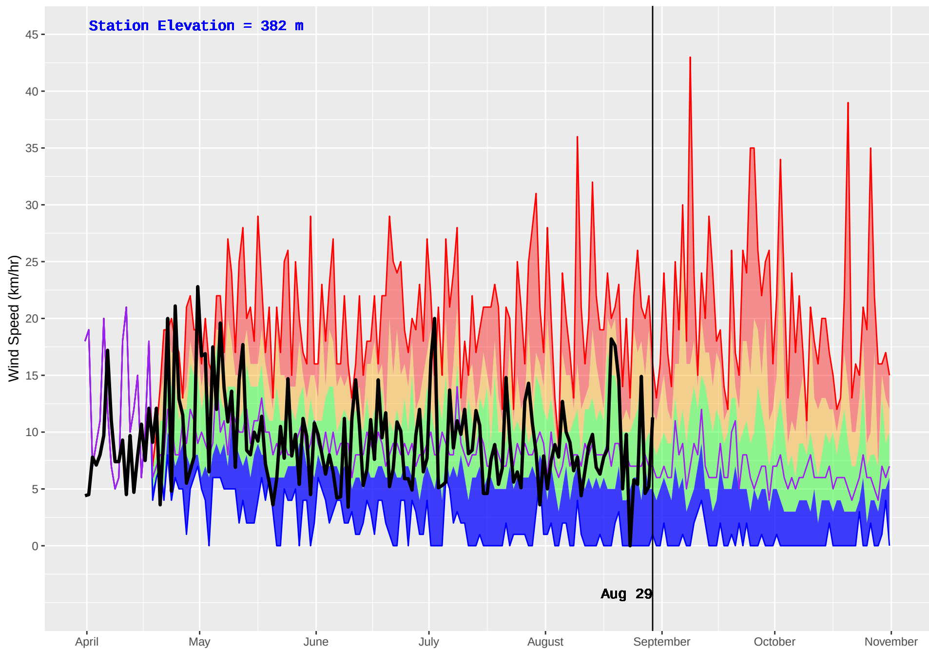
FORT NELSON FS (599) : Historical (1999–2016) and Current (2018) Daily Wind Speed
