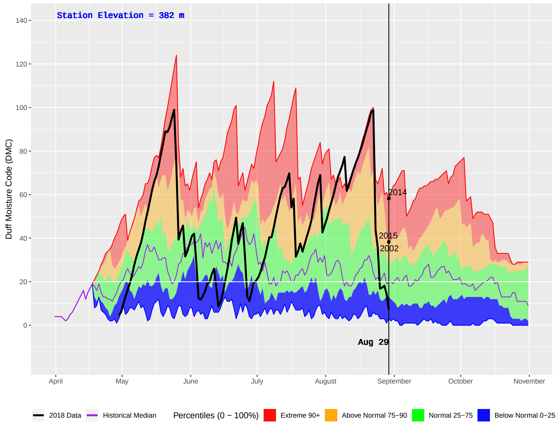
FORT NELSON FS (599) : Historical (1999–2016) and Current (2018) Daily Duff Moisture Code (DMC)
