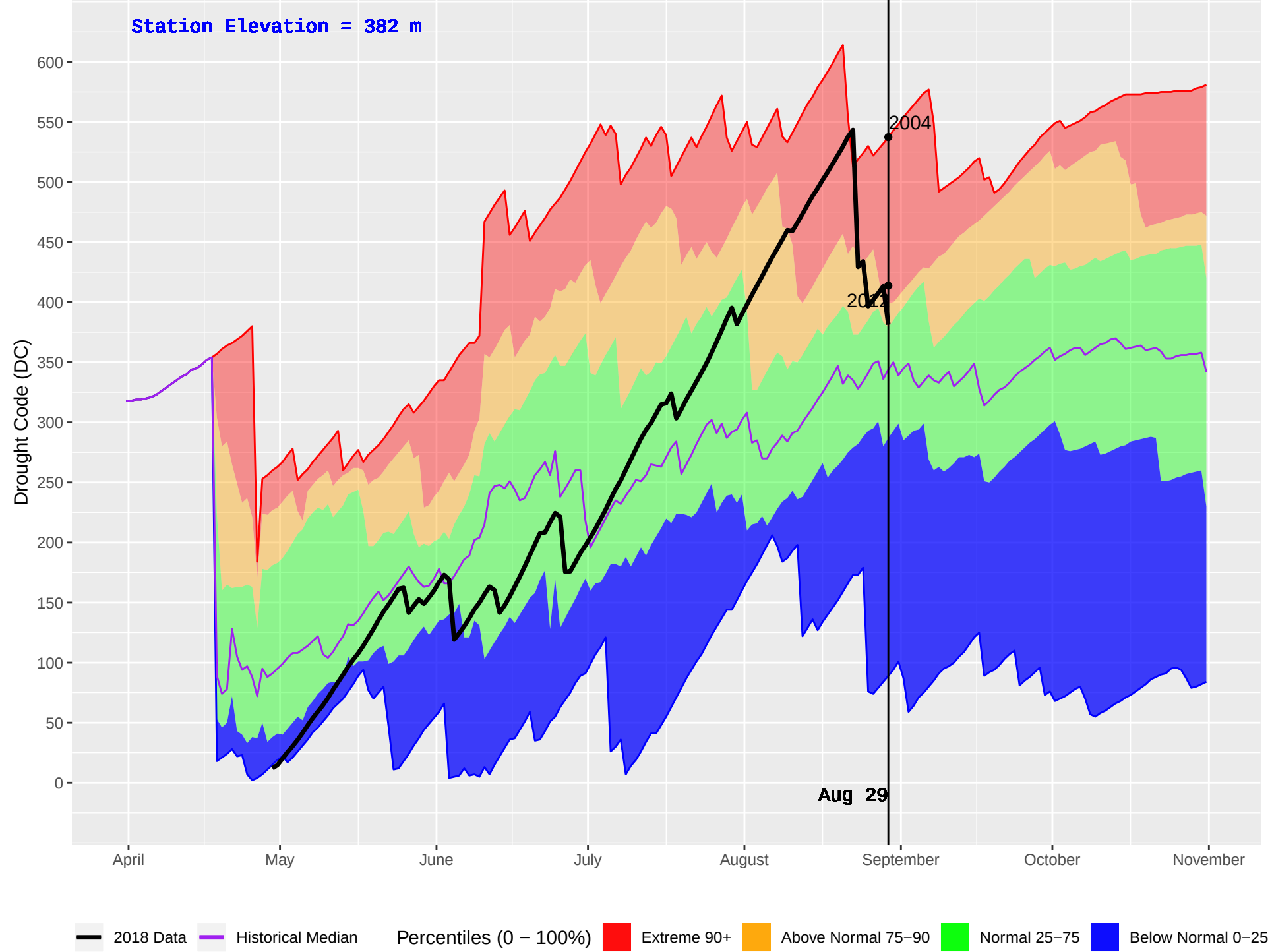
FORT NELSON FS (599) : Historical (1999–2016) and Current (2018) Daily Drought Code (DC)
