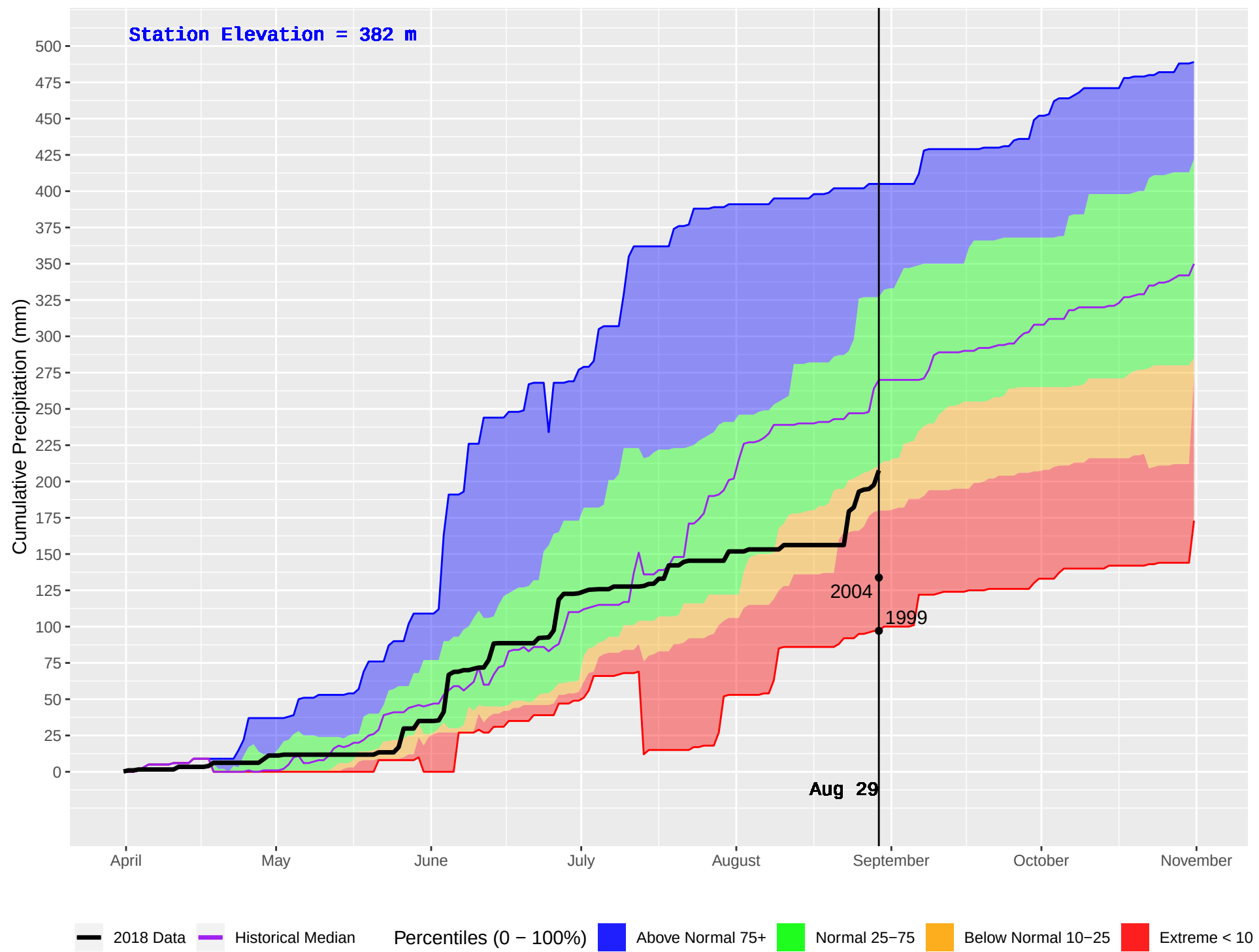
FORT NELSON FS (599) : Historical (1999–2016) and Current (2018) Daily Cumulative Precipitation
