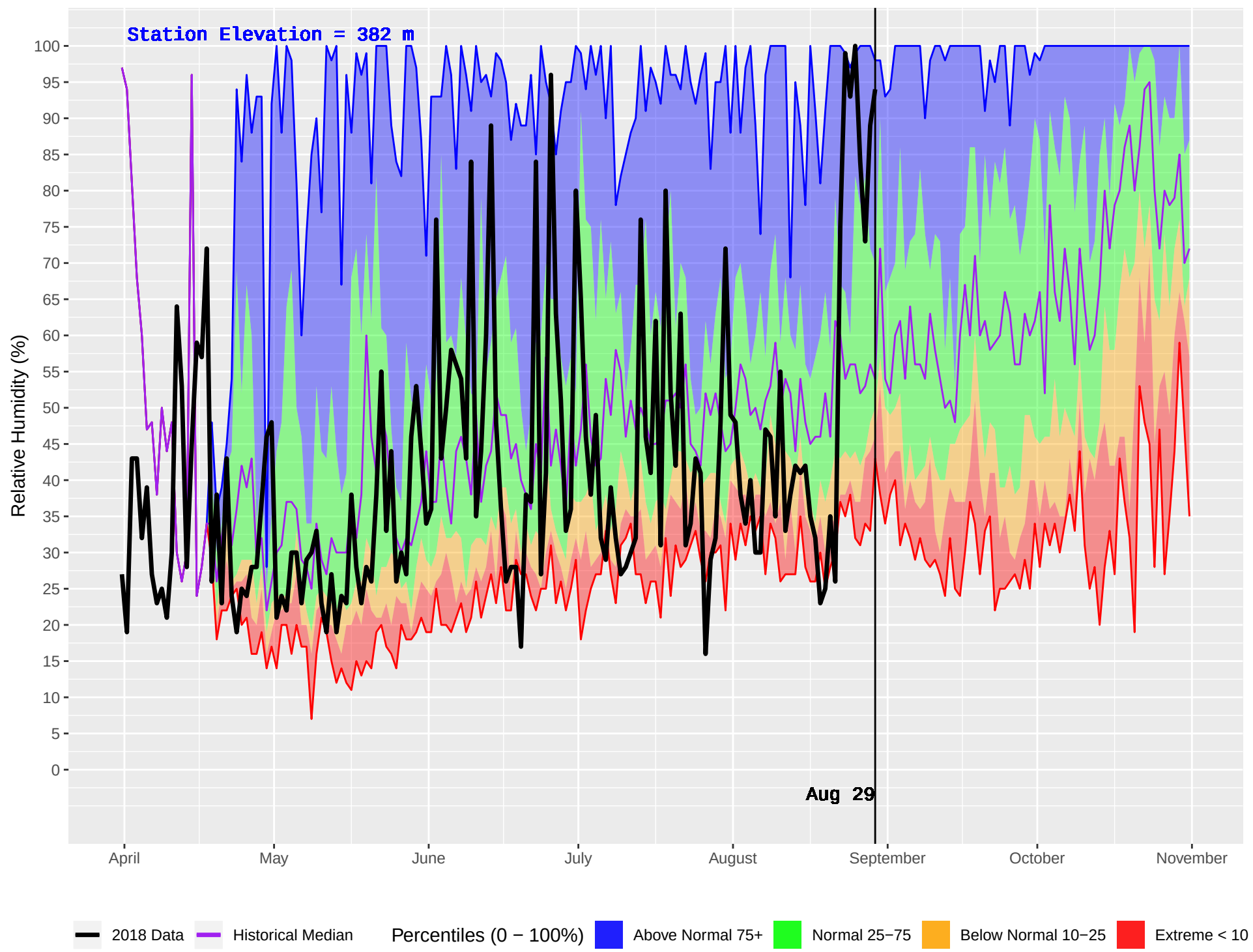
FORT NELSON FS (599) : Historical (1999–2016) and Current (2018) Daily Relative Humidity
