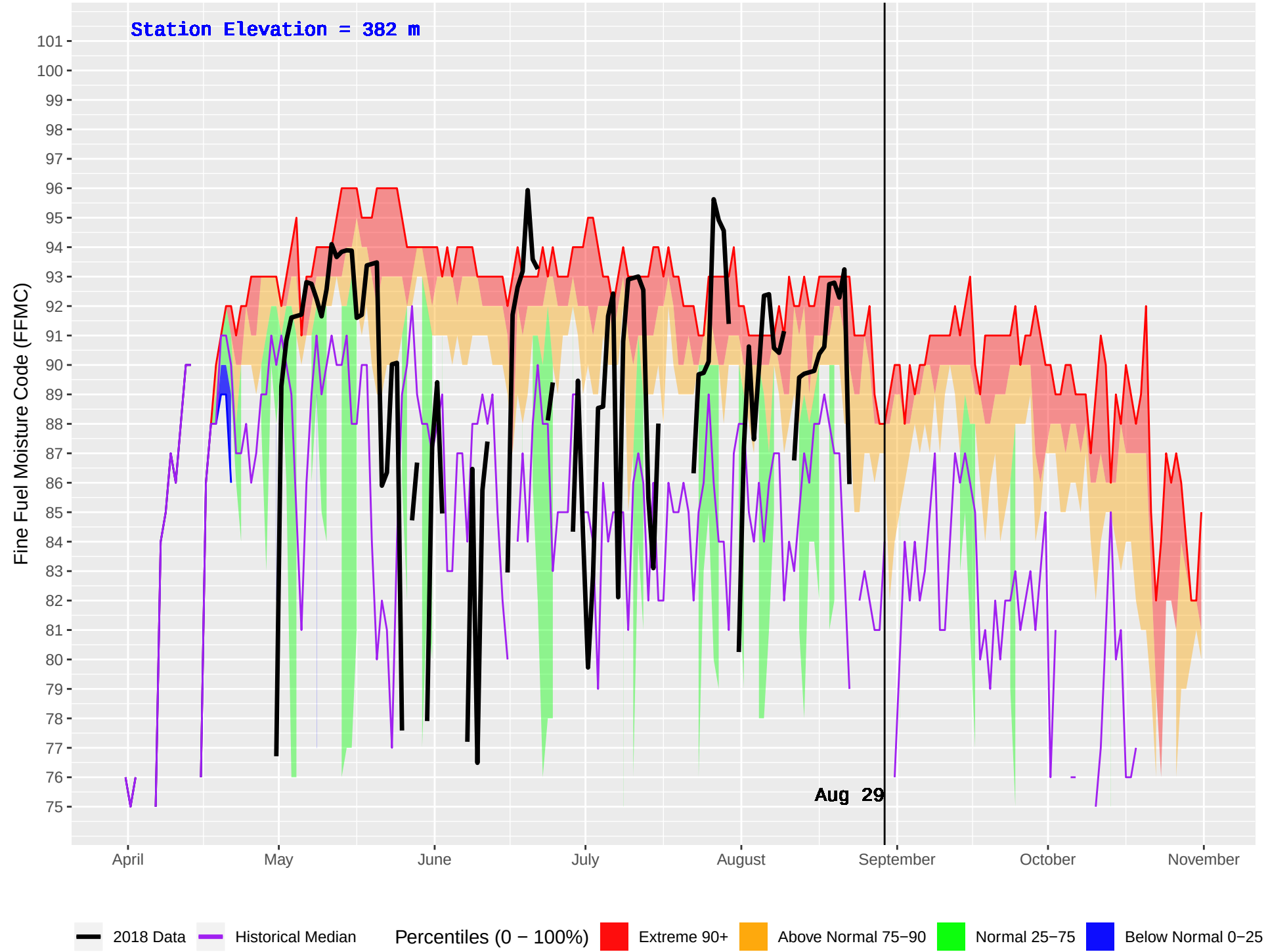
FORT NELSON FS (599) : Historical (1999–2016) and Current (2018) Daily Fine Fuel Moisture Code (FFMC)
