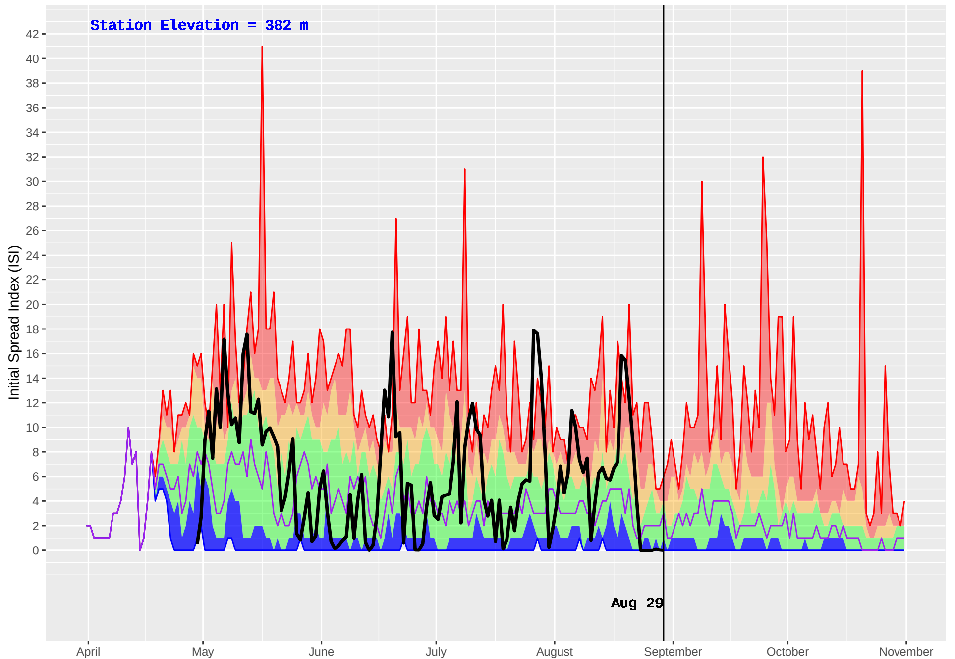
FORT NELSON FS (599) : Historical (1999–2016) and Current (2018) Daily Initial Spread Index (ISI)
