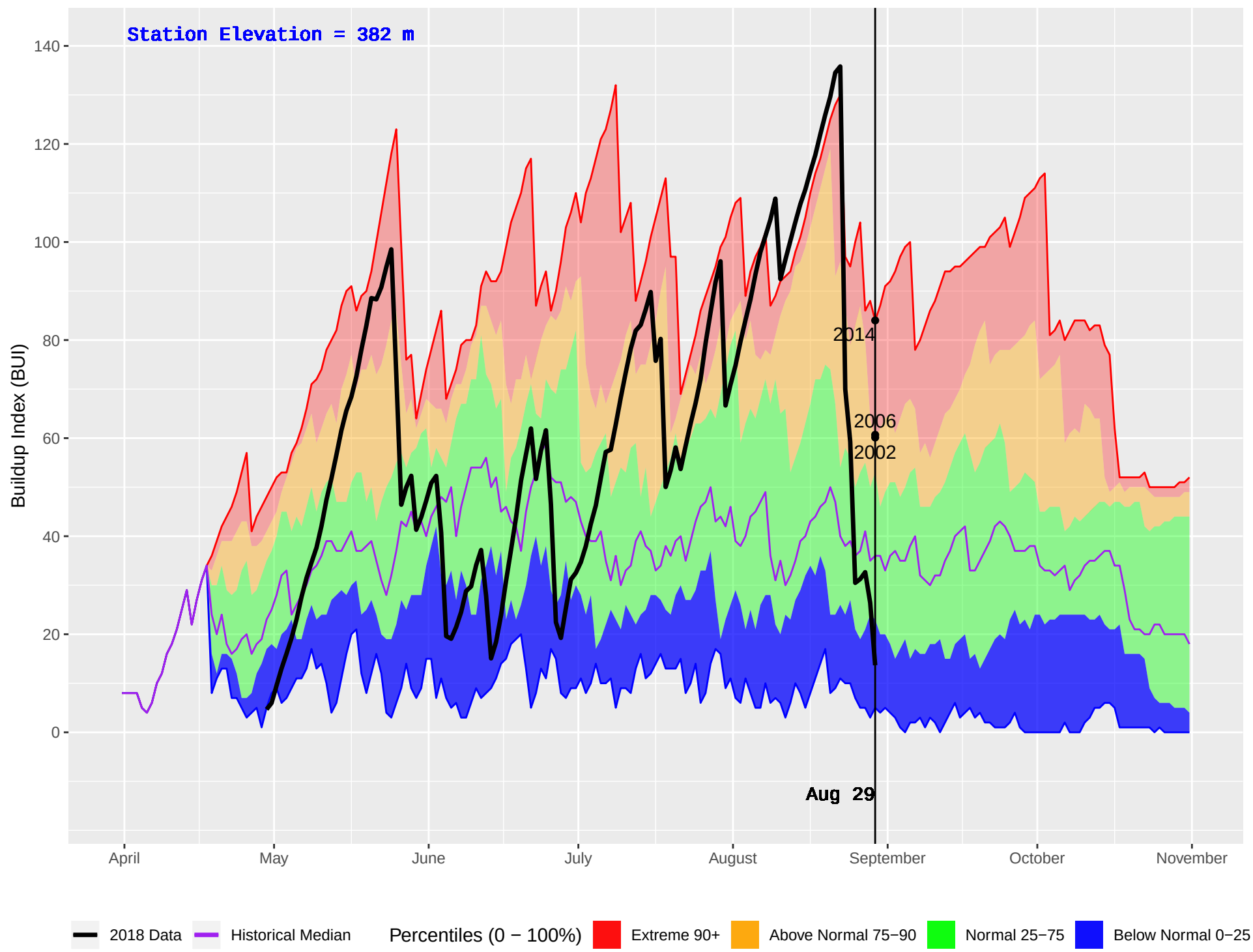
FORT NELSON FS (599) : Historical (1999–2016) and Current (2018) Daily Buildup Index (BUI)
